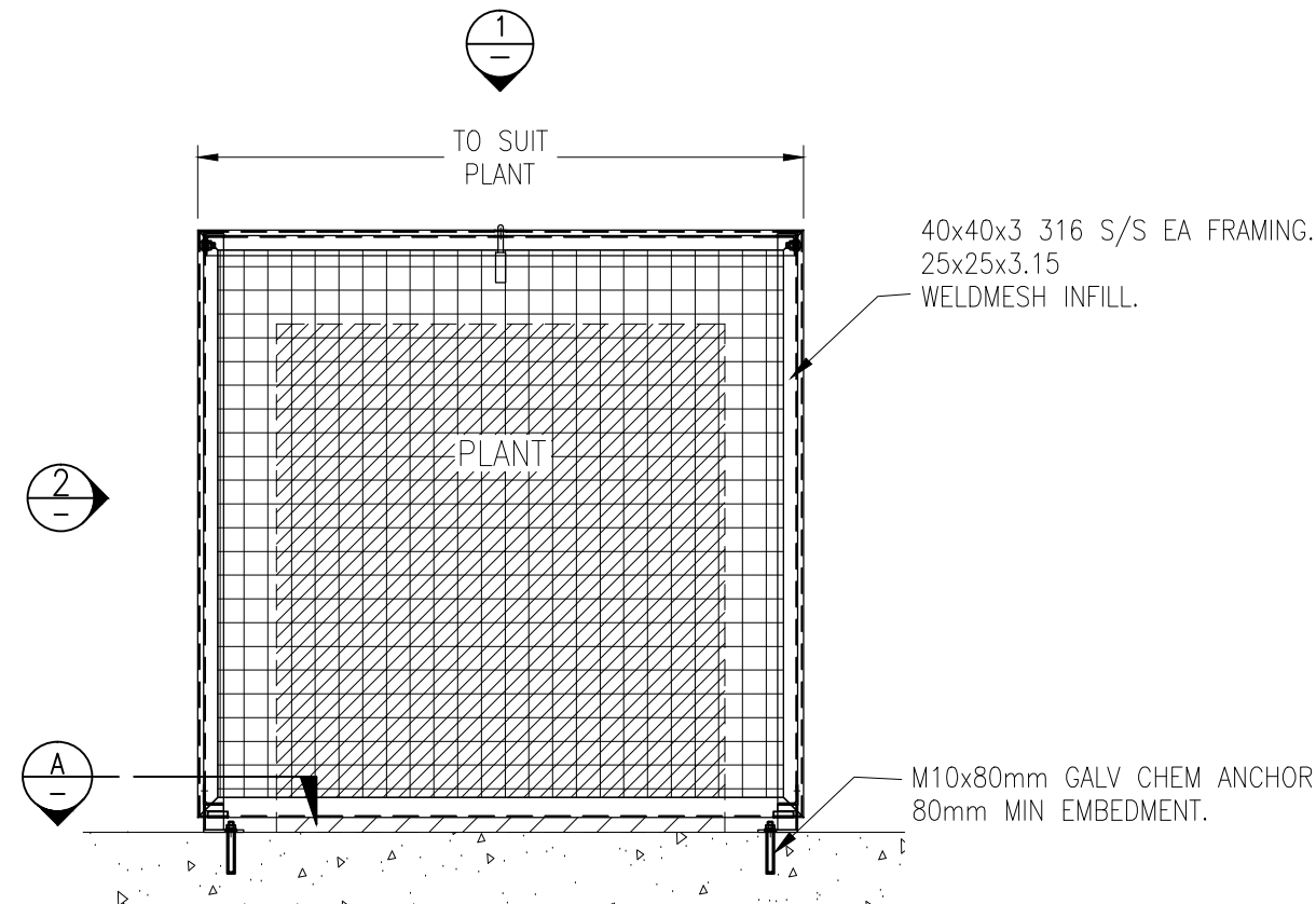
DETAIL E1 PLANT ENCLOSURE ELEVATION FABRICATED SIZE TO SUIT ORDER 40x40x3 316 S/S EQUAL ANGLE FRAME 25x25x3.15 316 S/S WELDMESH REMOVE ALL SHARP EDGES. M10 CHEM/MECH ANCHORS
