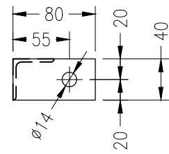
VIEW NTS A BASE PLATE DETAIL 5mm BASE PLATE FIX WITH M10 CHEM/MECH ANCHOR TYPICAL DETAIL
